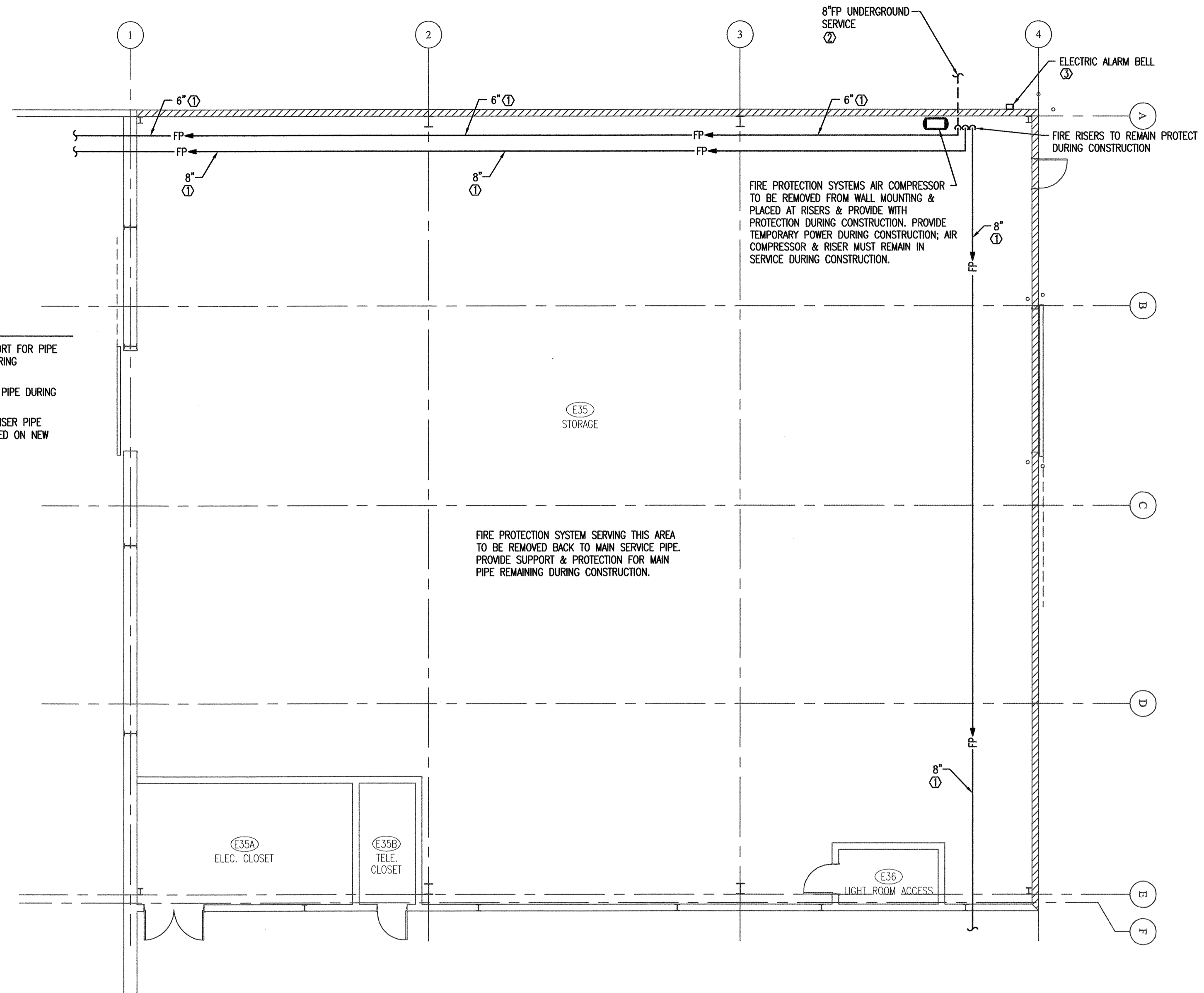
1 FIRE PROTECTION DEMOLITION FLOOR PLAN F2.01 SCALE: 1/8" = 1'-0"
