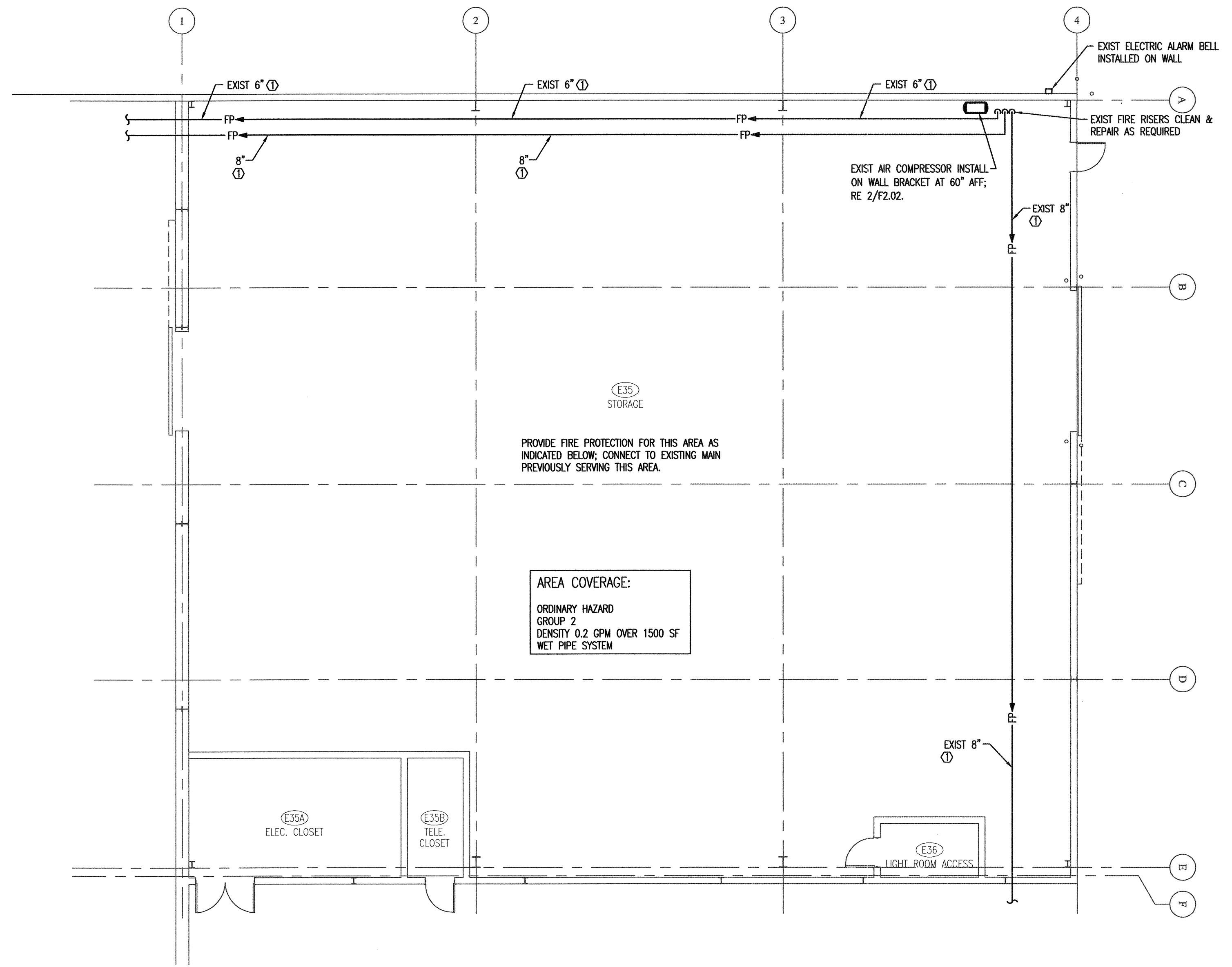
1 FIRE PROTECTION FLOOR PLAN F2.02 SCALE: 1/8" = 1'-0" N
