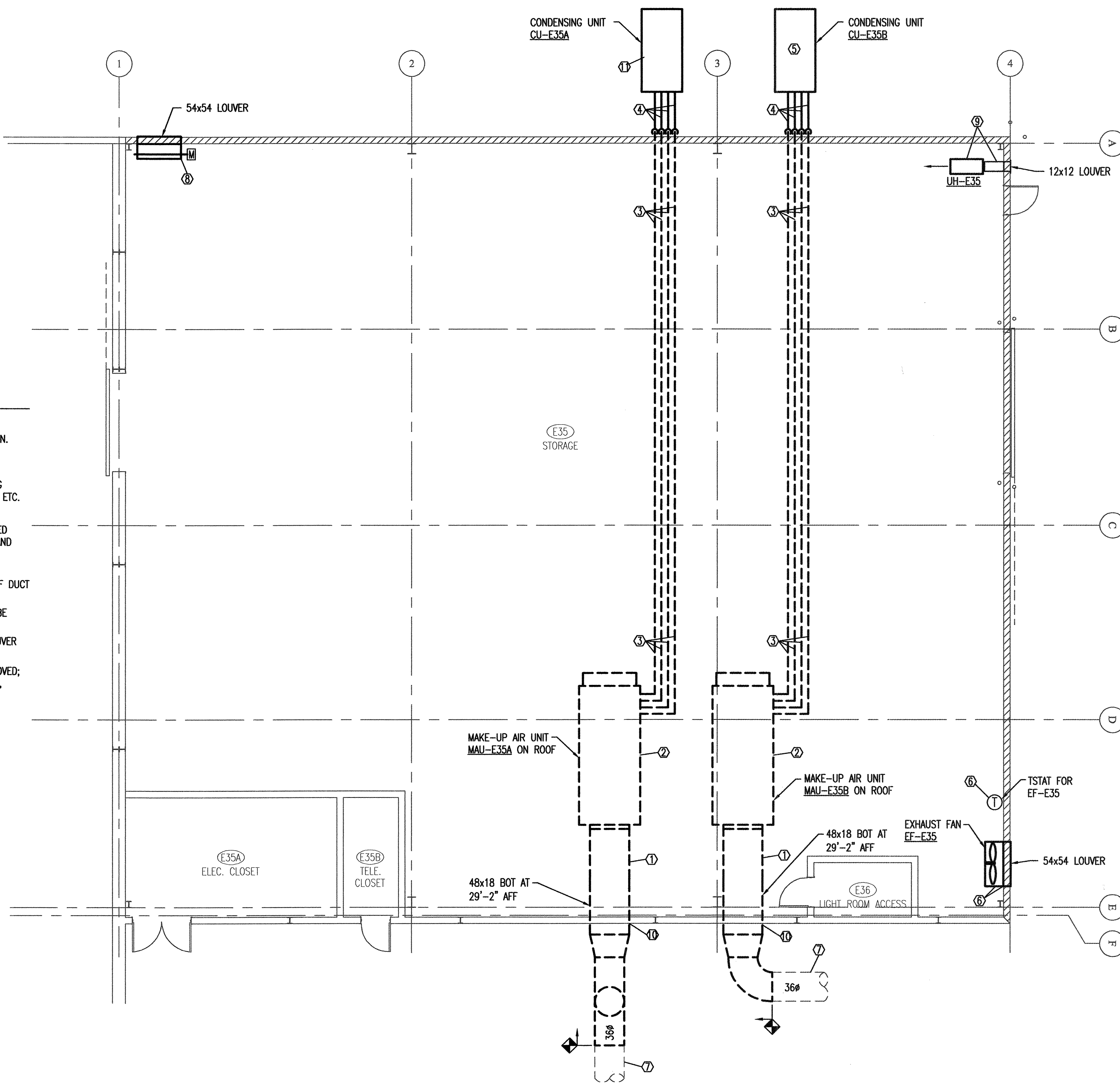
1 MECHANICAL DEMOLITION FLOOR PLAN M2.01 SCALE: 1/8" = 1'-0"
