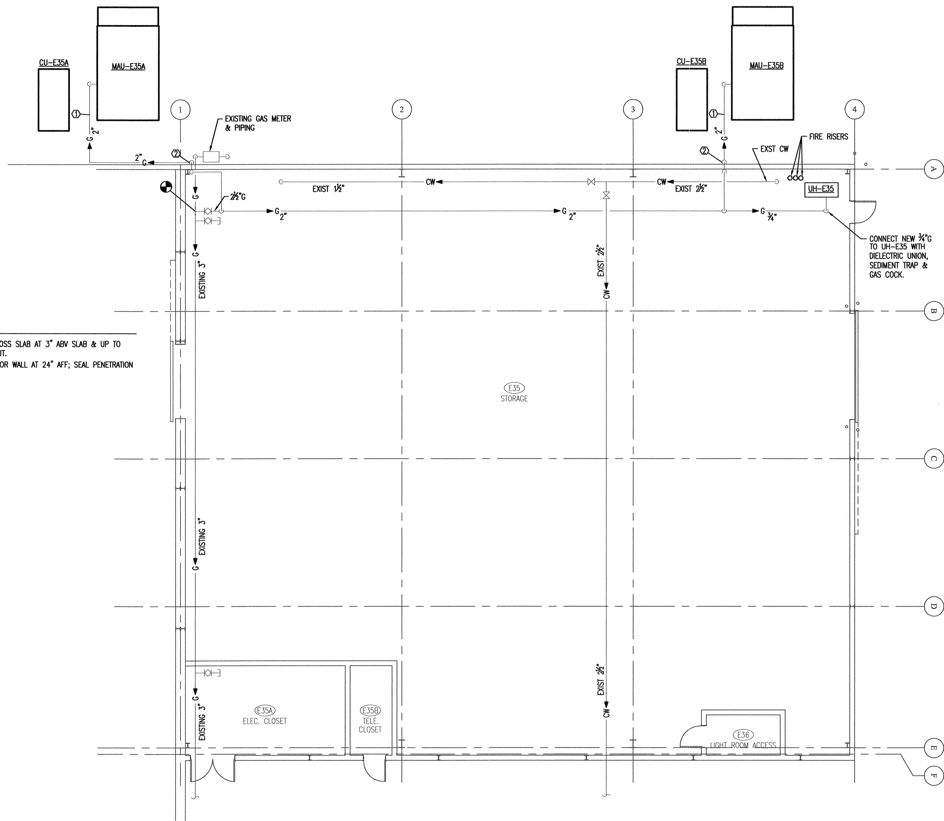
1 PLUMBING FLOOR PLAN P2.02 SCALE: 1/8" = 1'-0"
